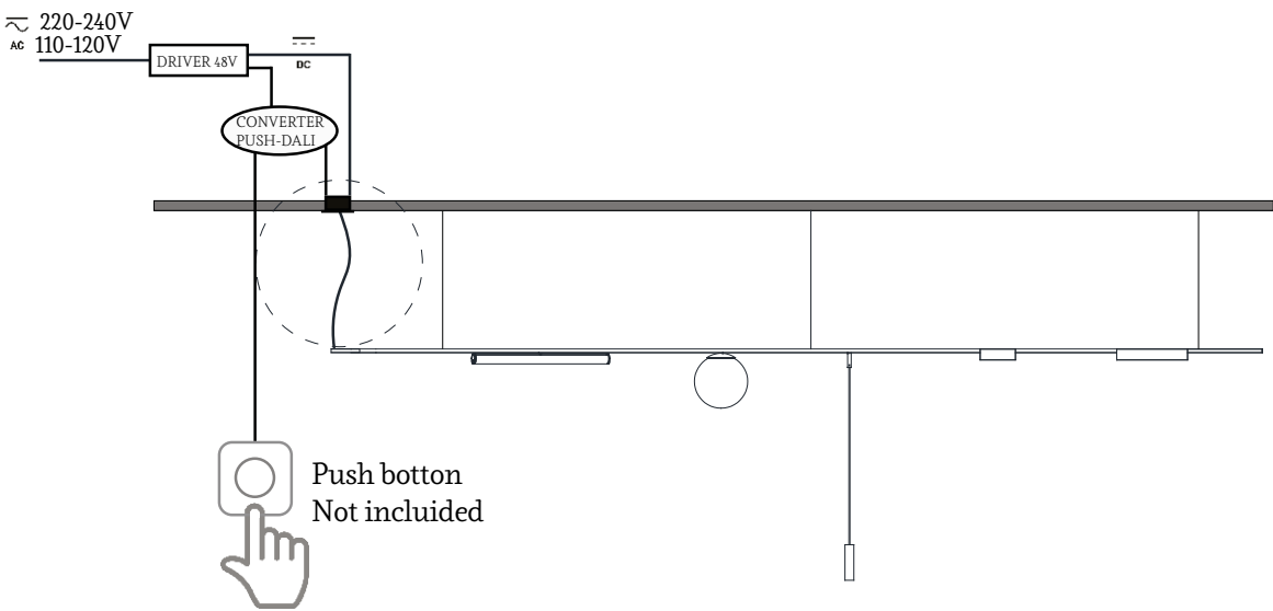
OPTION 5 - BLOKINLINE SYSTEM CANOPY SR 48V 120W DIM PUSH
