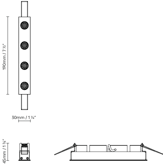
BLOKINLINE MODULE 4 RECESSED
