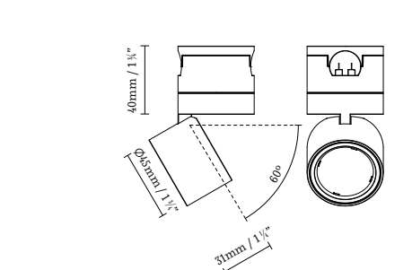
SIS SYSTEM SPOTLIGHT
