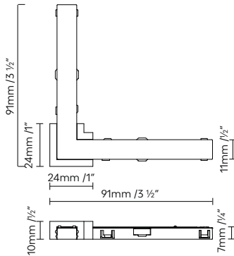
BLOKINLINE SYSTEM 90° H UNION
