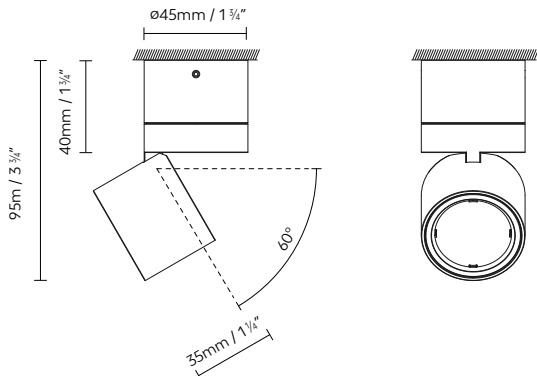
SIS SPOTLIGHT C D40
