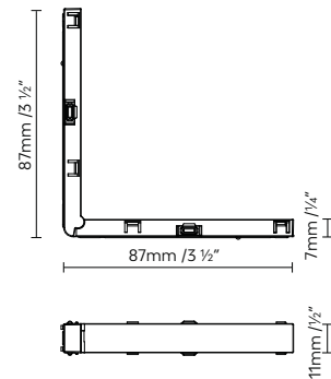
BLOKINLINE SYSTEM 90° V UNION
