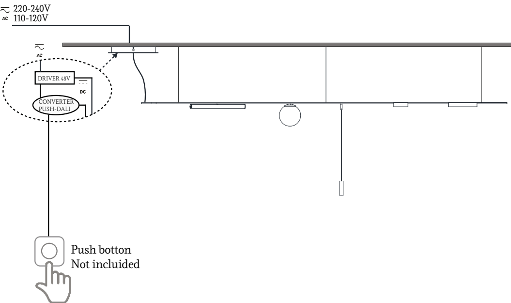
OPTION 3 - BLOKINLINE SYSTEM CANOPY S 48V 120W DIM PUSH
